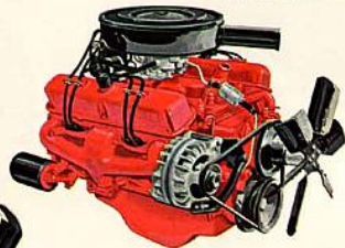
Optional V-8—318-cu.-in. 8-cylinder, 2-barrel carburetor, standard cam, single exhaust, 9.0 to 1 compression ratio, air cleaner with silencer, regular fuel.
