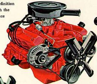
Optional V-8—318-cu.-in. 8-cylinder, 2-barrel carburetor, standard cam, single exhaust, 9.0 to 1 compression ratio, air cleaner with silencer, regular fuel.
