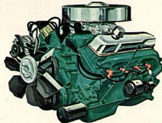
Optional High Performance Commando V-8—426-cu.-in. 8-cylinder, 4-barrel carburetor, special cam, dual exhaust, 10.3 to 1 compression ratio, unsilenced air cleaner, premium fuel.
