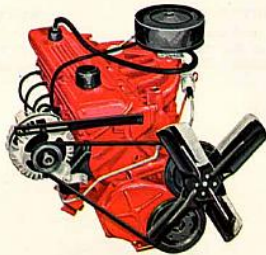
Standard Six—225-cu.-in. 6-cylinder, single-barrel carburetor, standard cam, single exhaust, 8.4 to 1 compression ratio, regular fuel.
