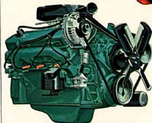
Optional High Performance Commando V-8—383-cu.-in. 8-cylinder, 4-barrel carburetor, special cam, dual exhaust, 10.0 to 1 compression ratio, unsilenced air cleaner, premium fuel.
