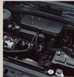
Acclaim's standard 2.5-liter dual balance- shaft EFI four-cylinder engine. Underhood service points are clearly labeled for easy maintenance.
