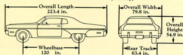
Dimensions Exterior 2-Door V-8 (Hardtop)
