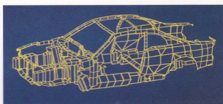
Super-monocoque body frame
