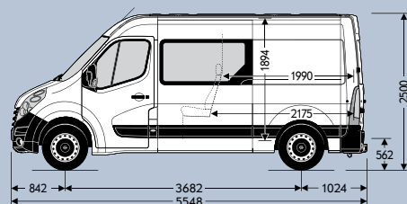
L2H2 traction
