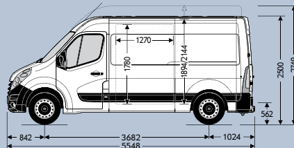
L2H2/H3 traction
