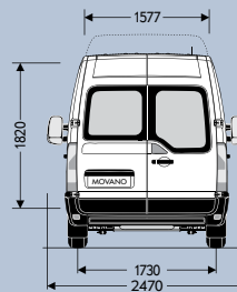
H2/H3 traction
