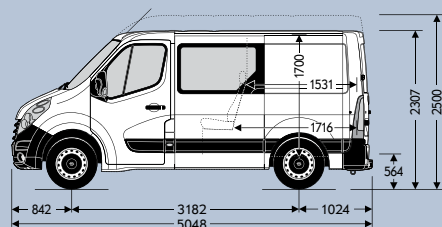
L1H1/H2 traction
