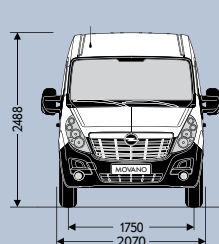
L3H2 traction
