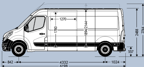
L3H2/H3 traction
