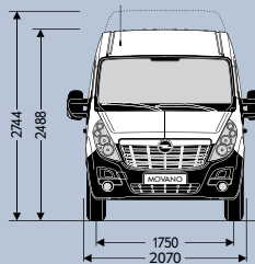
L3H2/H3 traction
