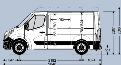
L1H1/H2 traction
