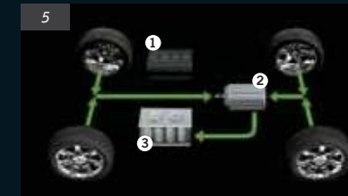
FIG. 5: REGENERATIVE BRAKING
