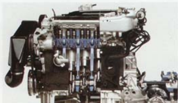
Powerful acceleration is ensured with maximum torque of 309Nm already being delivered at 1950 rpm.
