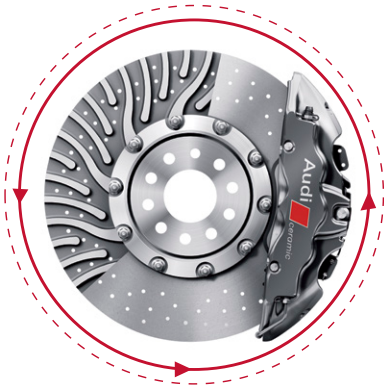
carbon ceramic rotor 1 // reduces rotational weight by up to 8.82 lb each
