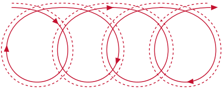
rotational momentum
