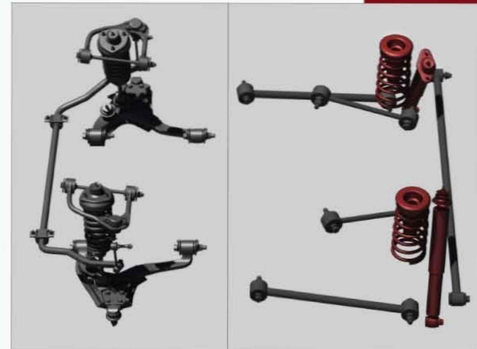
Independent Double Wishbone Front Suspension
