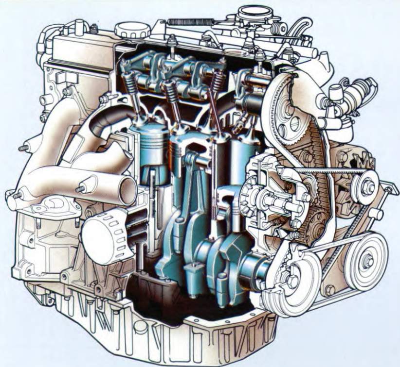
1995 cm 3 motor
