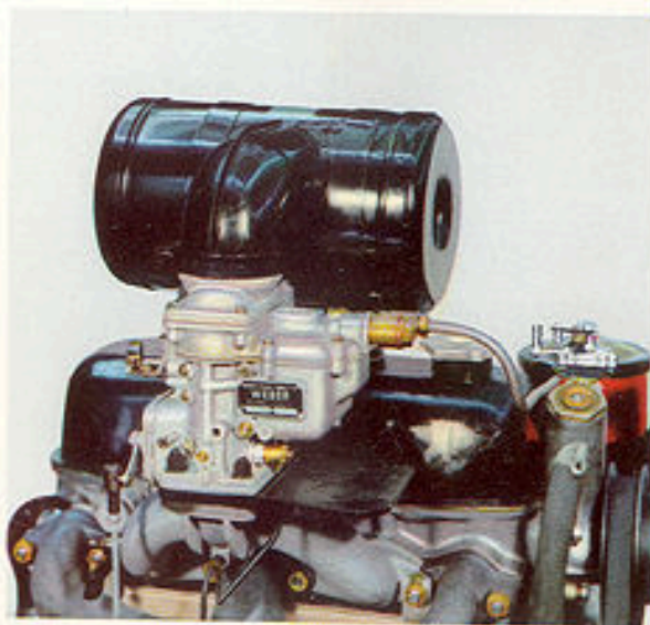
The "1100 TV" has a twin-body carburetter.
