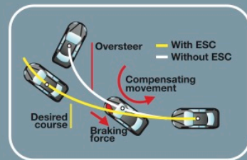
ELECTRONIC STABILITY CONTROL WITH BRAKE ASSIST
