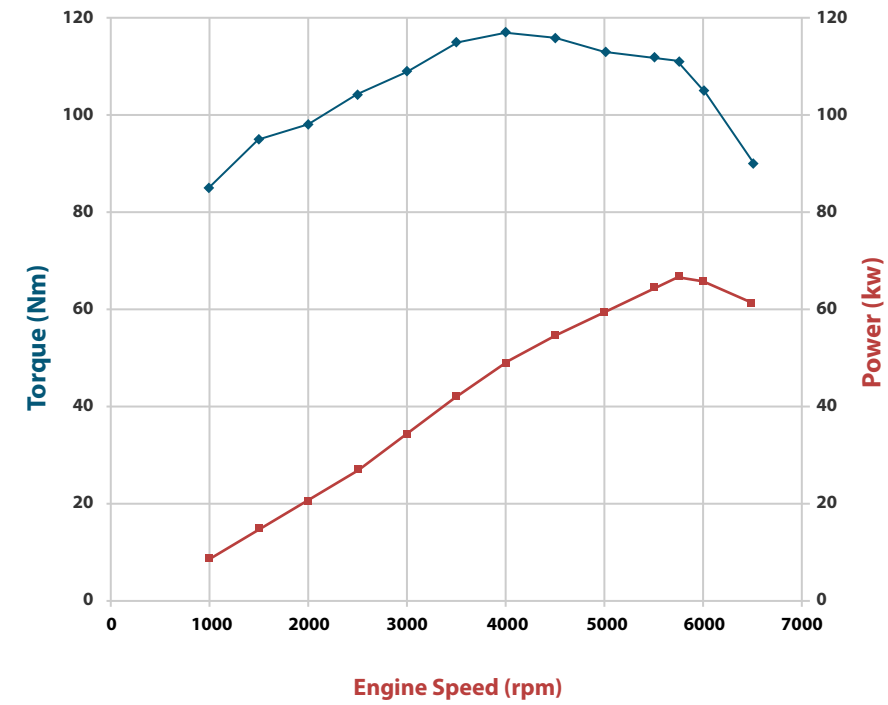
FULL LOAD PERFORMANCE CURVE FOR VVT 1299CC
