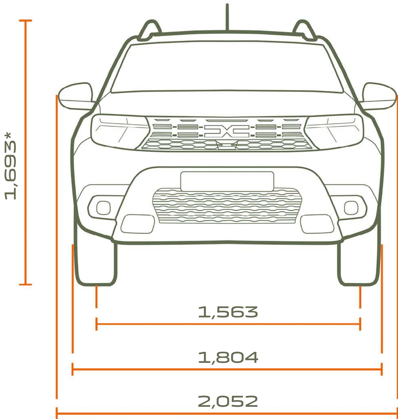
FRONT VIEW
