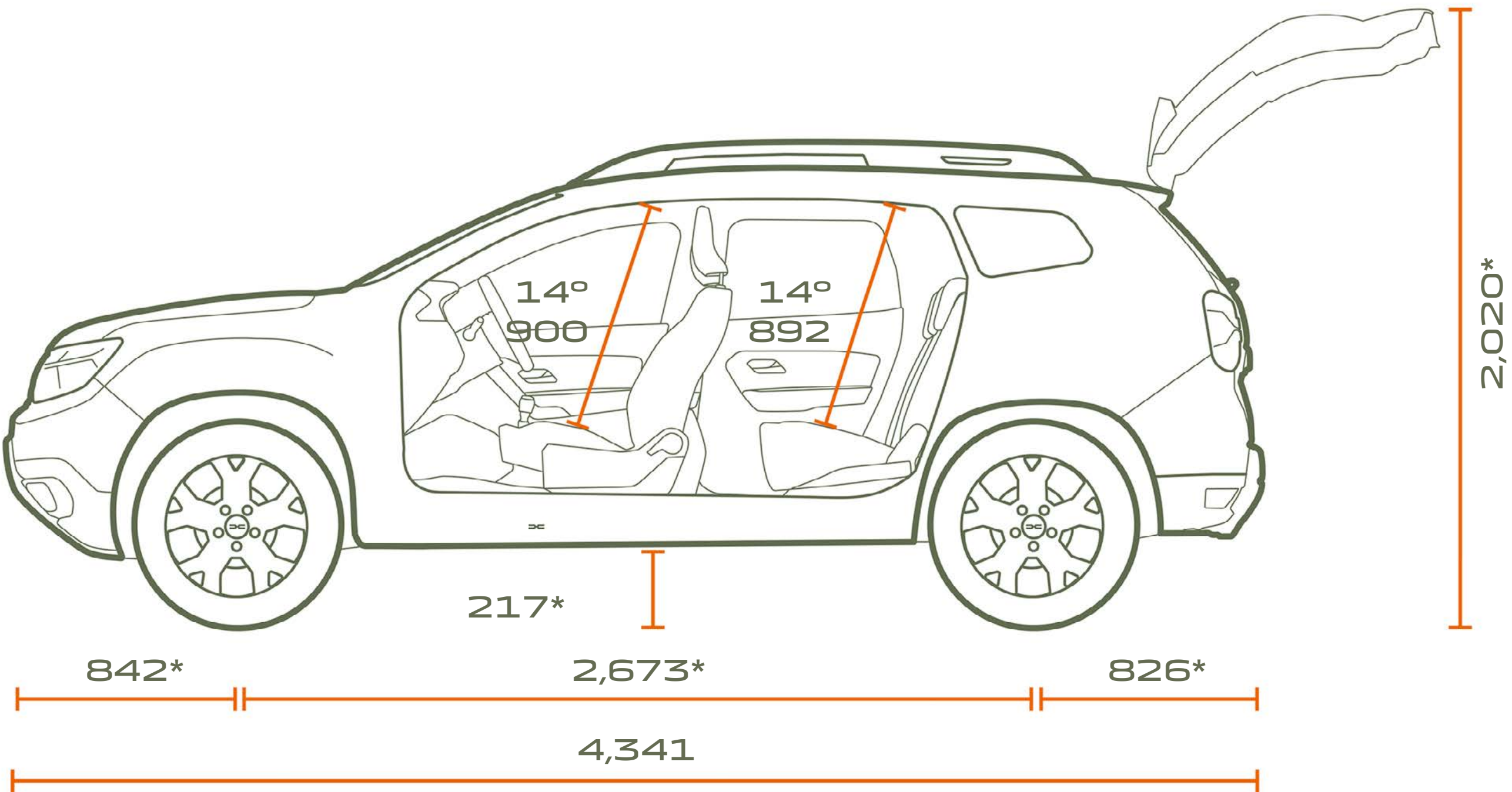
PROFILE VIEW
